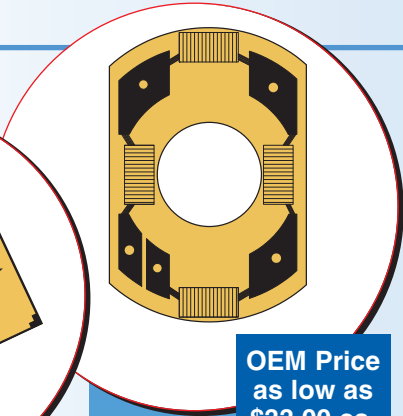
Custom Disc Gage Full Bridge Design SGC-1/350-1762
